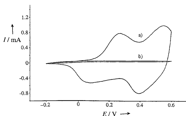
Figure 5. Cyclic voltammograms of a) the polyaniline-coated CP–NT coaxial nanowires and b) the bare aligned carbon nanotubes. Measured in an aqueous solution of 1M \text{H}_2\text{SO}_4 with a scan rate of 50 \text{ mV s}^{-1} .
